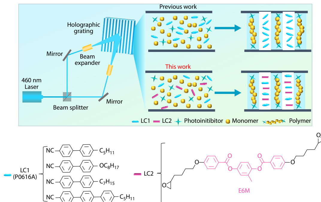
Fig. 1 Schematic illustration on the construction of high-performance LC-based holographic polymer nanocomposites by doping E6M. P0616A was commercially available LC in nematic phase.
